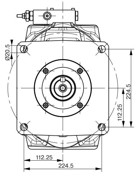
Mounting option E splined shaft 15T-8/16 DP, flat root, side fit ANSI B92.1
