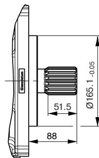
Output: splined shaft W50x 2 x 24 x 9 g DIN 5480
